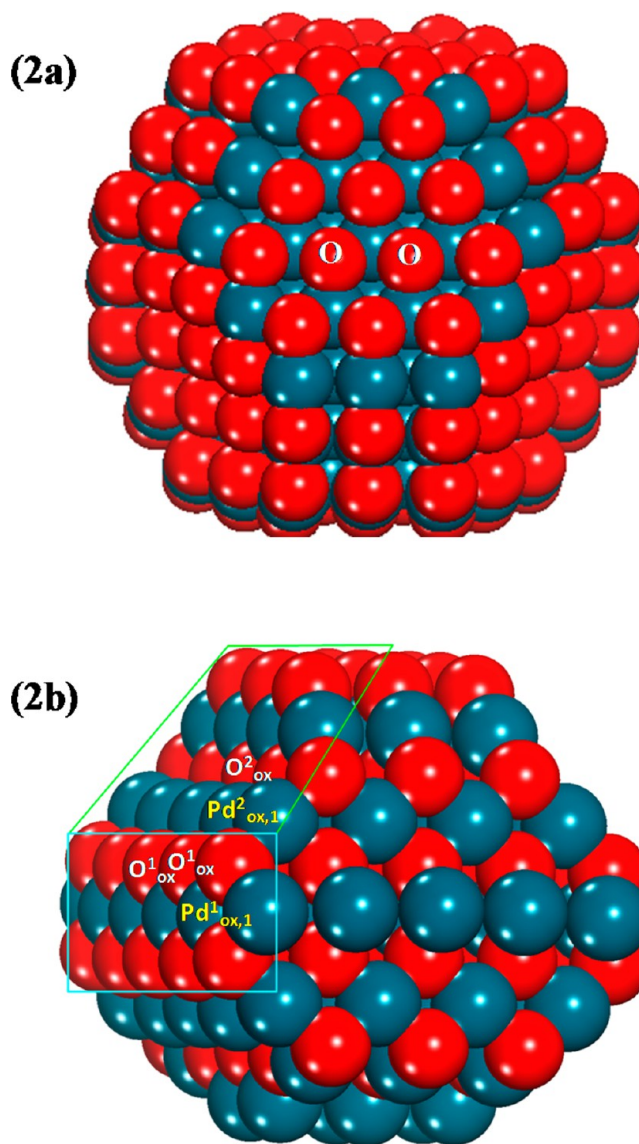
Figure 2. DFT-optimized model of cuboctahedral 1 ML O*-covered Pd and PdO clusters used to examine the activation of methane. (a) 1 ML O*-covered Pd 201 and (b) 183 atom PdO (Pd 94 O 89 ) clusters. The Pd and O atoms are shown in blue and red, respectively. The (100) and (101) facets on Pd 94 O 89 cluster are highlighted in blue and green, respectively. The nonstoichiometric Pd ox –O ox (labeled Pd 1 ox,1 –O 1 ox ), the stoichiometric Pd ox –O ox (labeled Pd 2 ox,1 –O 1 ox ) and the O ox –O ox site pairs (labeled O 1 ox –O 1 ox ) are the only sites considered as the sites involving the four-coordinate O 2 ox sites are inaccessible. Note that O 1 ox atoms are shared between PdO(100) and PdO(101) facets.
